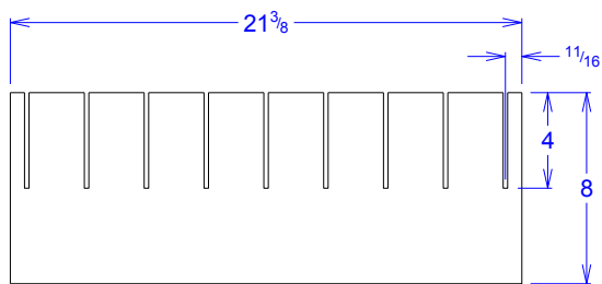
Part B Req 3 pcs
