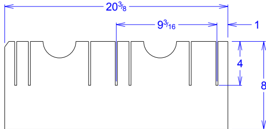
Part A Req 9 pcs
