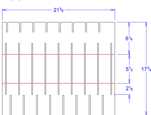
Part C Req 2 pcs
