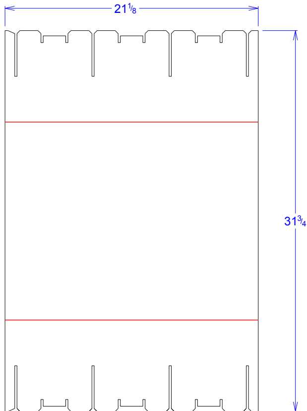
Part A Req 1 Pc
